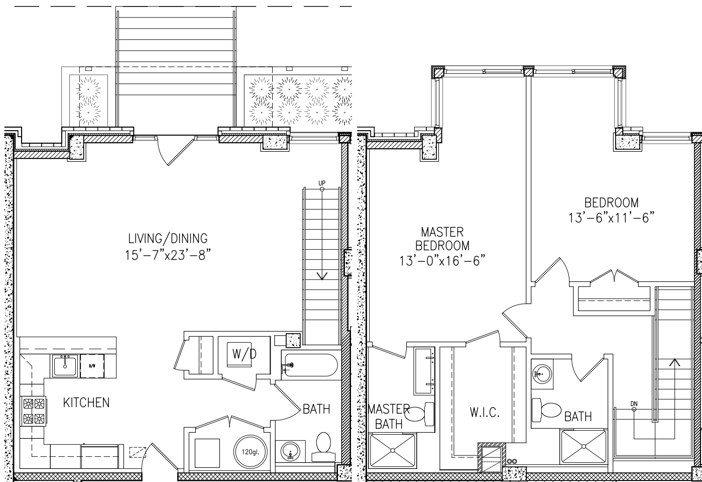
1ST FLOOR
